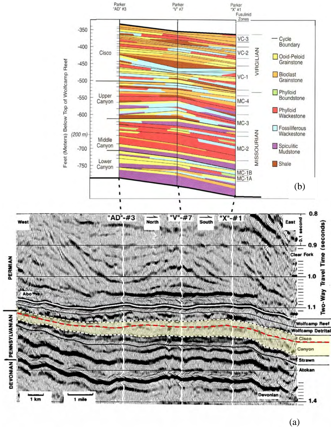
Figure 30. (a) Subregional seismic section of Southwest Andrews area. Yellow fill denotes Missouriian and Virgilian succession, with red dashes demarking the transition. Note that the seismic section is chairlike in reality, with wells V#7 and X#1 being equally basinward of AD3 along strike. (b) Facies reconstruction of Missouriian and Virgilian in the Southwest Andrews area. Refer also to comment above. After Saller and others (1999a, b).
