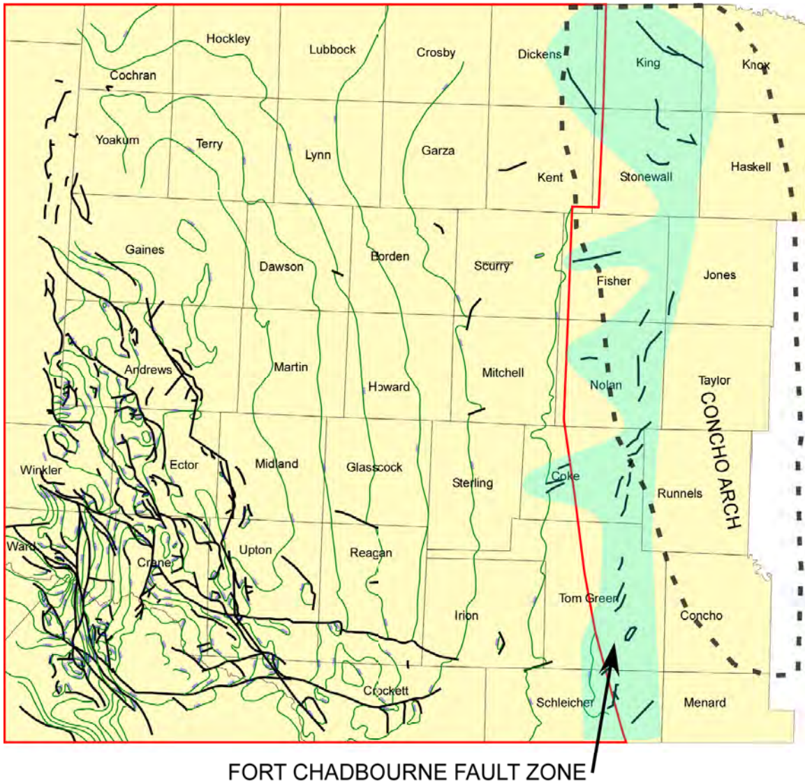
Figure 47. Regional structure map of Midland Basin. Green contour lines from top Ellenburger structure. Faults in black derived from Ewing (1983). Fort Chadbourne Fault Zone outlined in blue. Trend of Concho Arch indicated by dashed polygon. Strong correspondence between mid- to late Desmoinesian shelf margin and fault zone.
