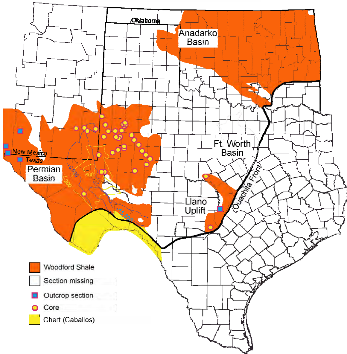
Figure 8. Example of distribution map (Woodford Formation).
