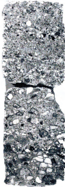
Upward-fining sequence in Atokan fan-delta from Standard and Robinson #2 Tippen well, Cottle Co.
