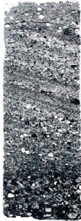
Crossbedding in Atokan fan-delta, from Standard Oil #1 Barron well, Cottle Co.
