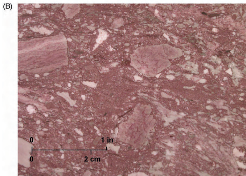
Figure 15. Artesia Group eolian sandstone and mixed sandstone/carbonate facies: (A) Yates uncommon, ripple-laminated, fine-grained sandstone from probable eolian setting (University No. 3210-2 well, Embar field, Andrews County) and (B) Yates dissolution-collapse-brecciated dolomite in siliciclastic matrix. Facies is similar to that found in dissolution zone depicted in figure 31 (HSA No. 1281 well, North Ward-Estes, Ward County).
