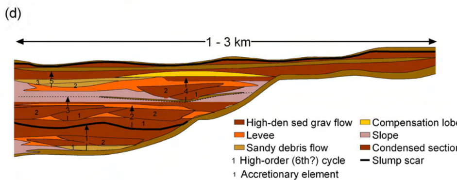
Figure 25. Brushy Canyon depositional cycle models of Gardner (1992): (a) processes during sea-level highstand include restriction of continental siliclastic depositional environments well shelfward of shelf margin, deposition in basin of windblown silt, and gravity transport of shelf-margin carbonate debris; (b) processes during sea-level lowstand include encroachment of prominently eolian depositional environments on shelf margin, accumulation of siliclastics on upper slope, slumping of accumulated siliclastics, and downslope transport of siliclastics by turbidity flow; (c) idealized model of relationship of channel-lobe complex to slump scar; and (d) idealized strike section showing depositional environments, slump scars, and depositional elements of high-order cycles. Slumping may place updip margins of reservoir facies in contact with low-permeability slope siltstones, thus providing updip lateral seal to some reservoirs.
