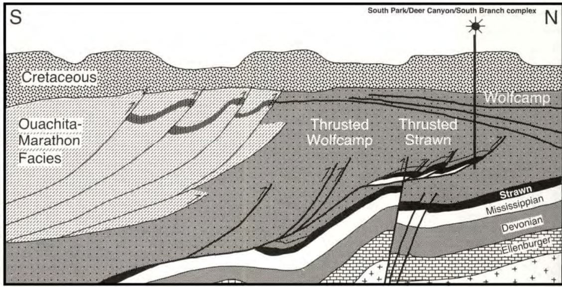
Figure 38. Schematic south-north diagram of Val Verde Basin thrust succession. After Newell and others (2003). There are two main thrust belts. The first contains thrusting of Mississippian, Strawn Formation, and Wolfcampian sediments and is termed the Foreland Thrust (fig. 36). The second is younger and contains Ouachita-Marathon siliciclastic facies and is termed the Ouachita Marathon Thrust.
